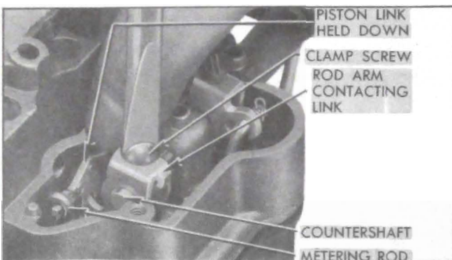
Figure 3-54—Metering Rod Adjustment
