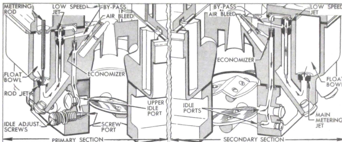
Figure 3-42—Primary and Secondary Low Speed Systems—WCFB Carter
