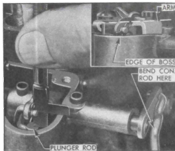
Figure 3-53—Checking Pump Plunger Adjustment
