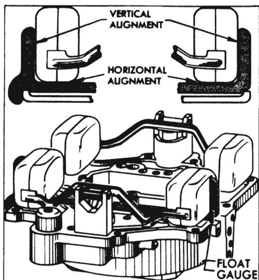
Figure 3-52—Checking Float Adjustment With Gauge
