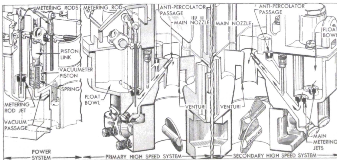
Figure 3-43—High Speed and Power Systems—WCFB Carter
