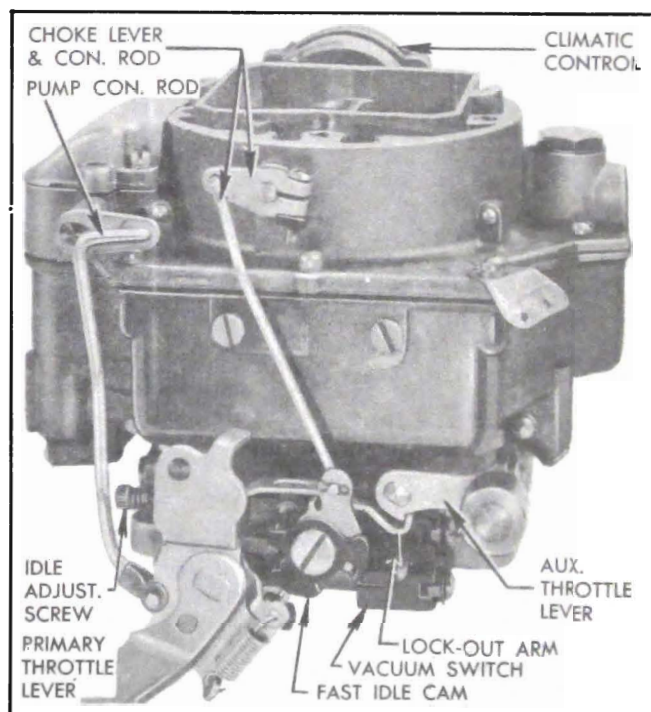
Figure 3-40—Carter WCFB Carburetor Assembly
