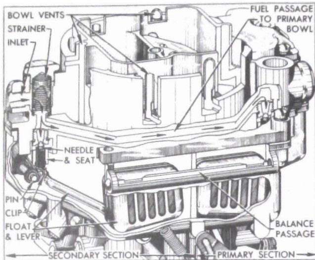
Figure 3-41—Primary and Secondary Float Systems—WCFB Carter
