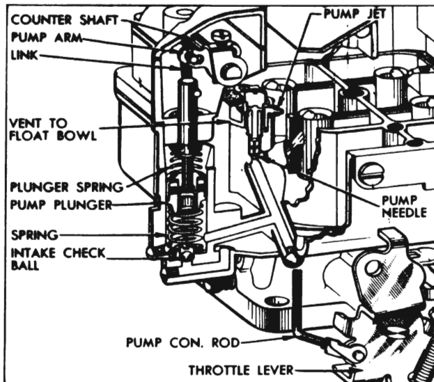
Figure 3-44—Accelerating System—WCFB Carter
