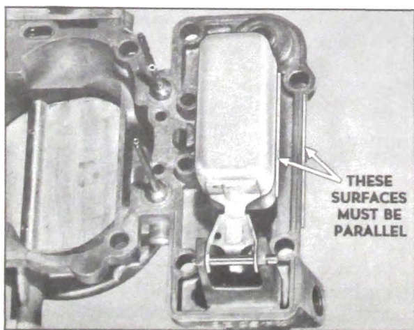
Figure 3-36—Checking Float Alignment
