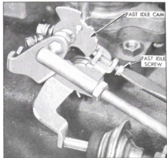
Figure 3-29—Adjusting Fast Idle Speed (on Engine)
