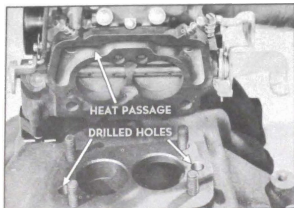
Figure 3-20—Exhaust Heat Passage
