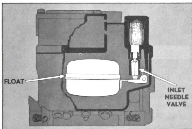
Figure 3-18—Float System
