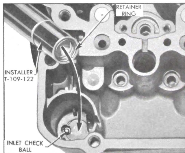
Figure 3-35—Installing Inlet Check Ball Retainer
