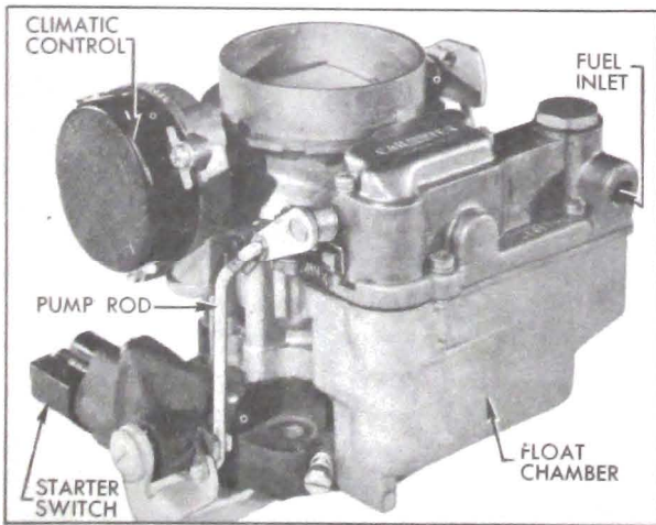
Figure 3-17—Carter WGD Carburetor Assembly
