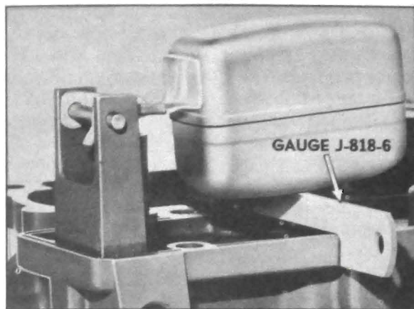
Figure 3-37—Checking Float Level
