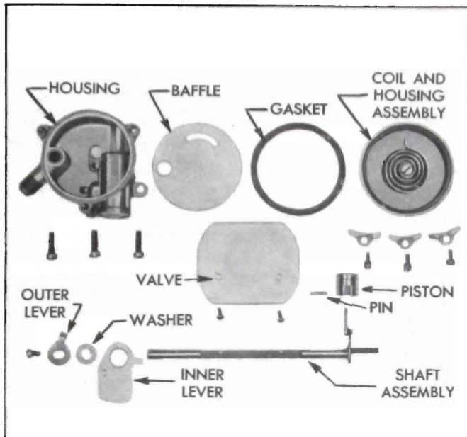
Figure 3-31—Climatic Control—Disassembled
