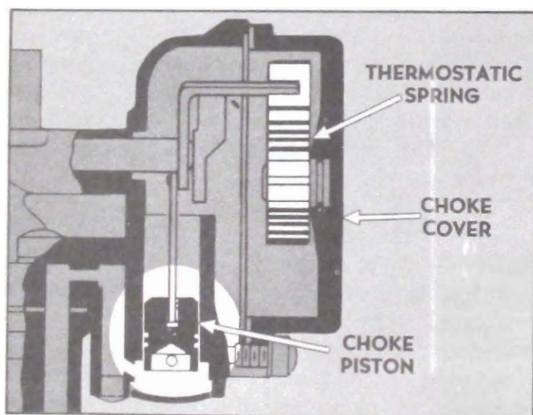
Figure 3-24—Climatic Control
