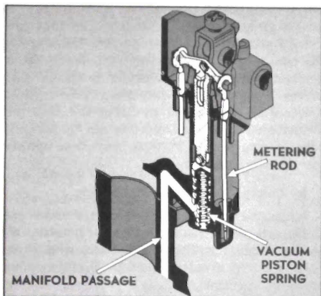
Figure 3-22—Power System
