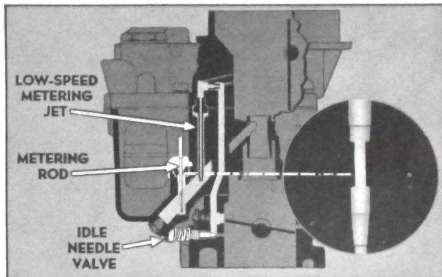
Figure 3-19—Low Speed System
