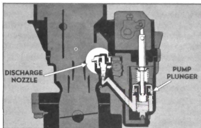
Figure 3-23—Accelerating System
