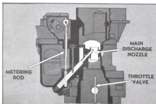
Figure 3-21—High Speed System
