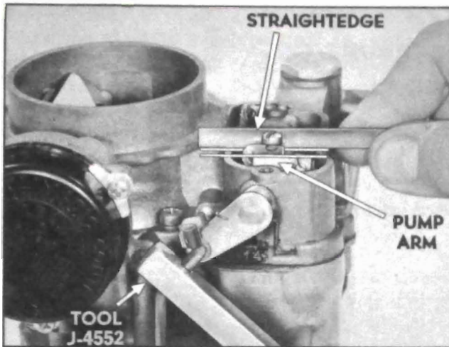
Figure 3-38—Checking and Adjusting Pump
