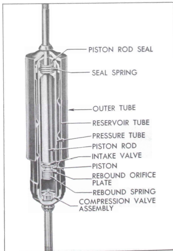
Figure 7-4—Front Shock Absorber—Sectional View
