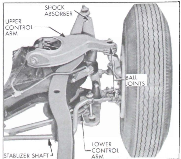
Figure 7-1—Front Wheel Suspension
