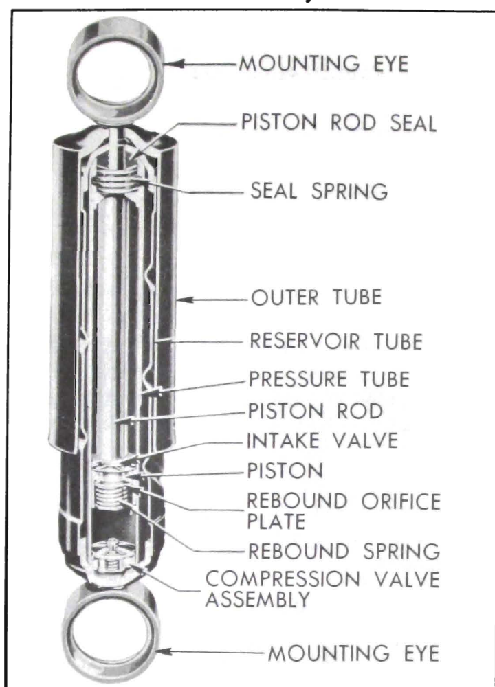
Figure 7-5—Rear Shock Absorber—Sectional View
