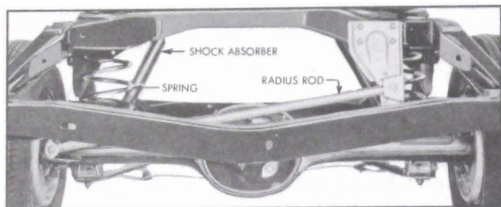
Figure 7-3—Rear Wheel Suspension
