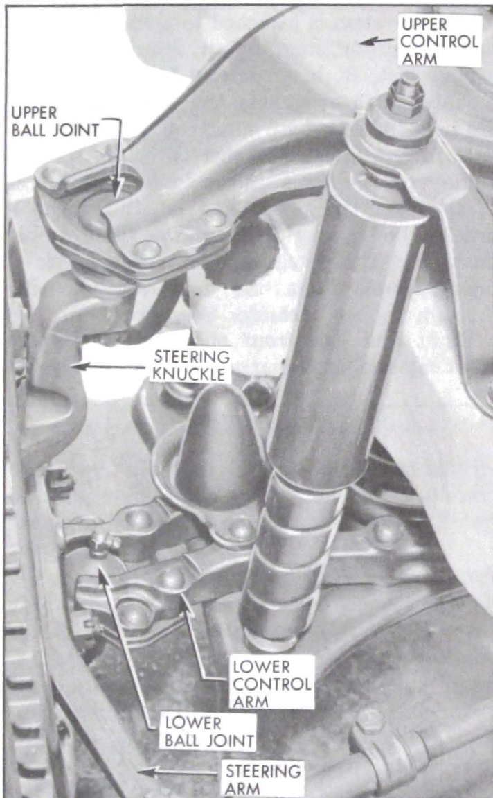
Figure 7-2—Left Steering Knuckle and Ball Joints
