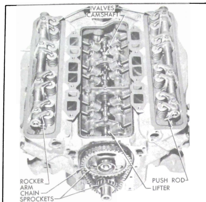
Figure 2-8—Valve Mechanism
