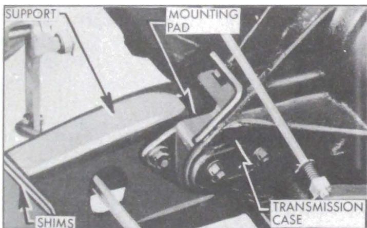
Figure 2-4—Triple Turbine Mounting
