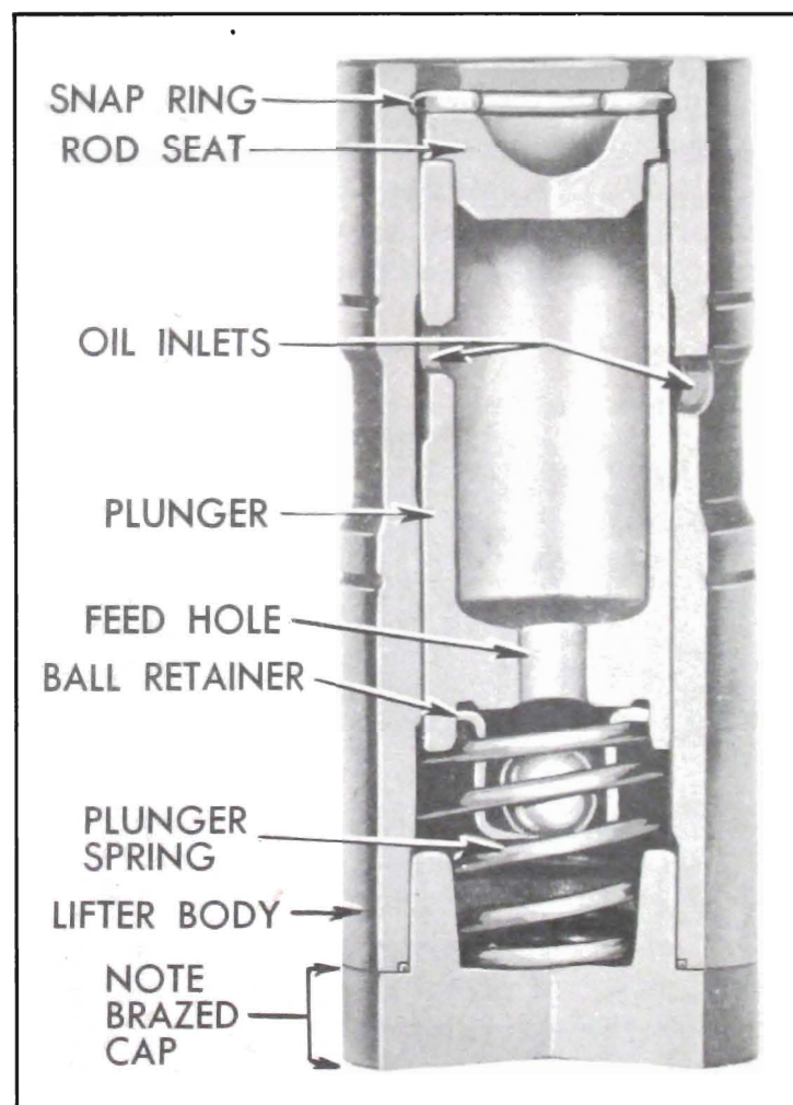
Figure 2-9—Hydraulic Valve Lifter, Sectional View
