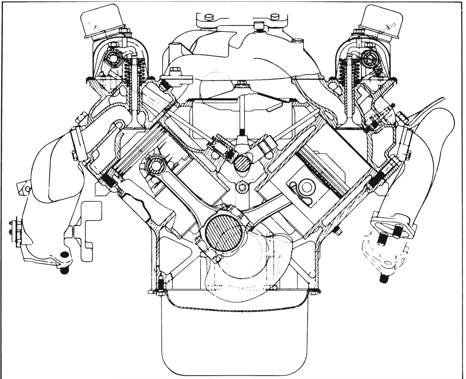
Figure 2-1—Engine End Sectional View
