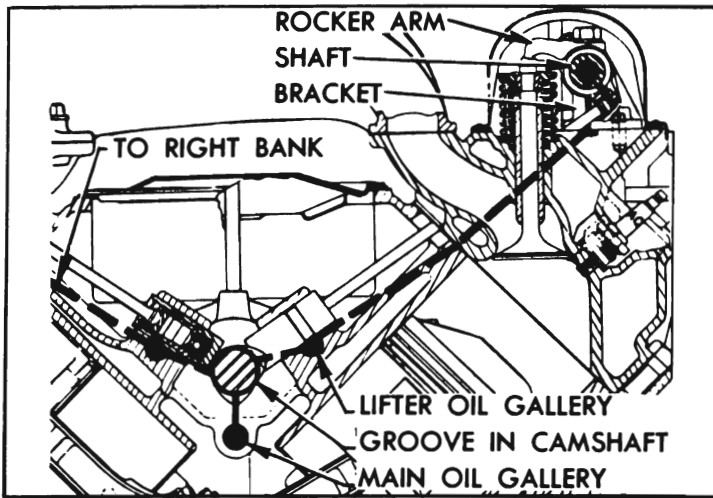
Figure 2-12—Oil Supply to Lifters, Rocker Arms and Valves
