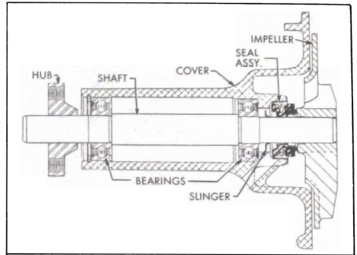
Figure 2-15—Water Pump Cover Assembly
