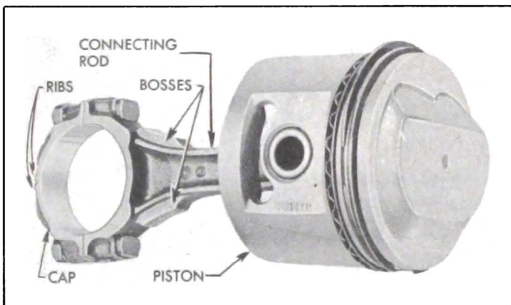
Figure 2-7—Connecting Rod and Piston Assembly
