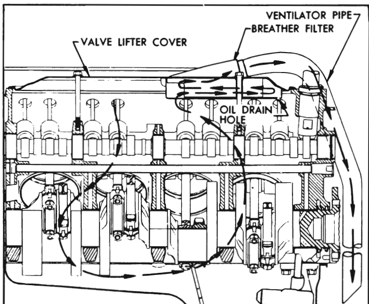
Figure 2-13—Crankcase Ventilation
