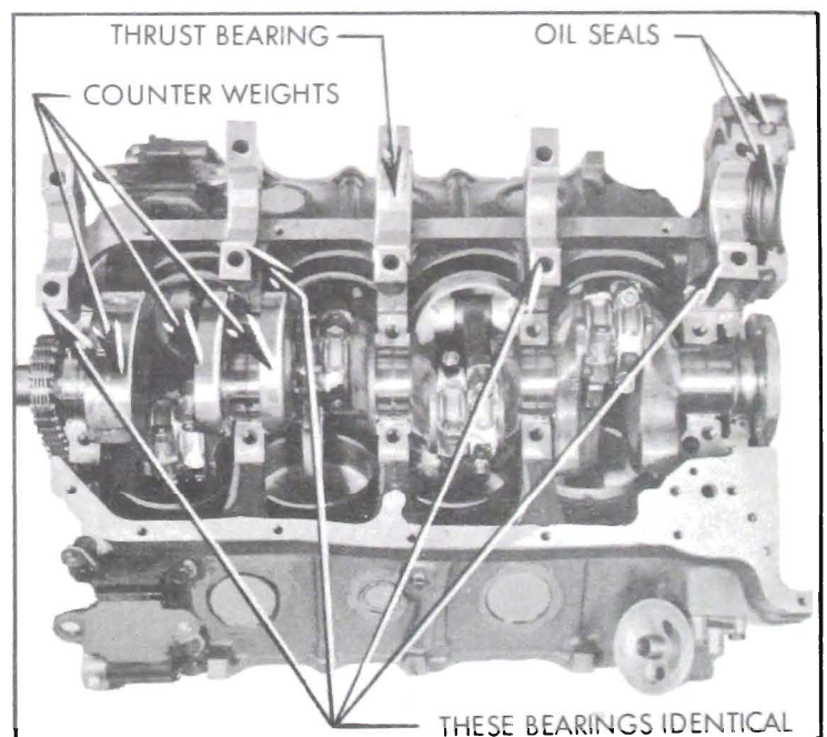
Figure 2-6—401 Engine Crankshaft and Bearings
