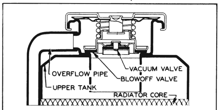
Figure 2-14—Pressure Type Radiator Cap Installation
