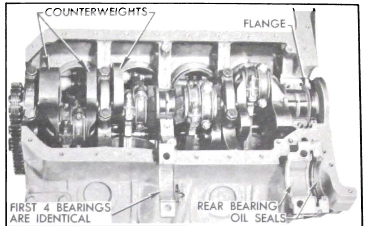
Figure 2-5—364 Engine Crankshaft and Bearings
