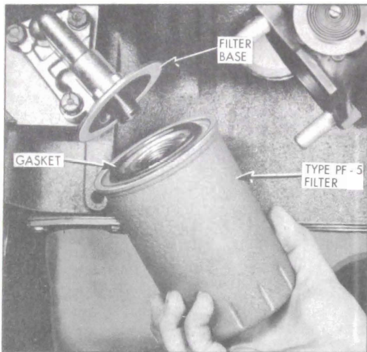
Figure 2-10—Oil Filter Installation
