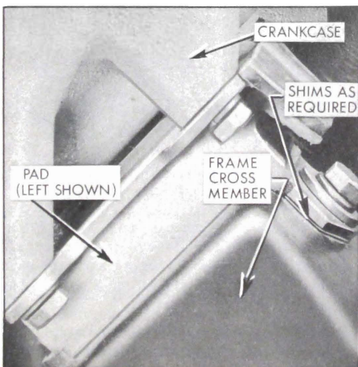
Figure 2-2—Front Engine Mounting
