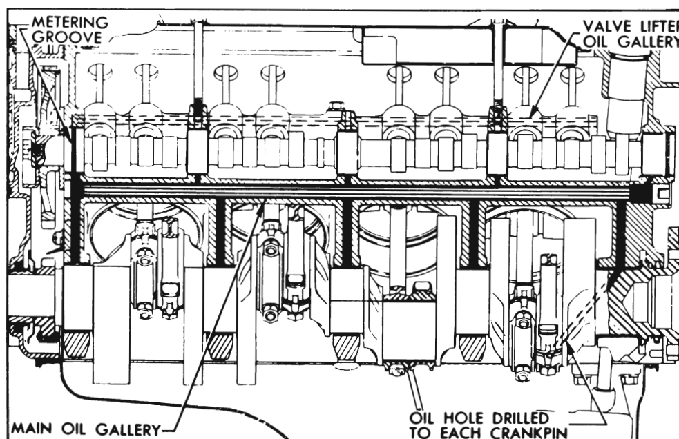
Figure 2-11—Oil Galleries—364 Engine Shown
