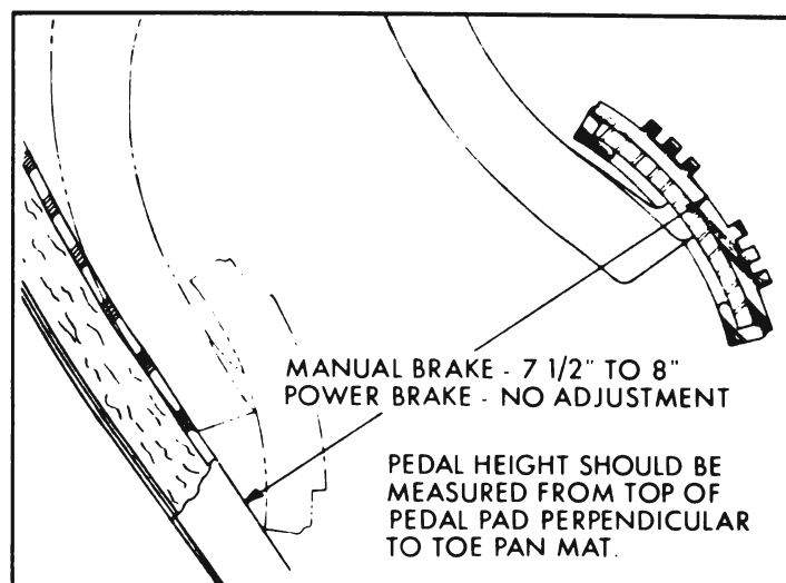
Figure 9-7—Brake Pedal Height Adjustment
