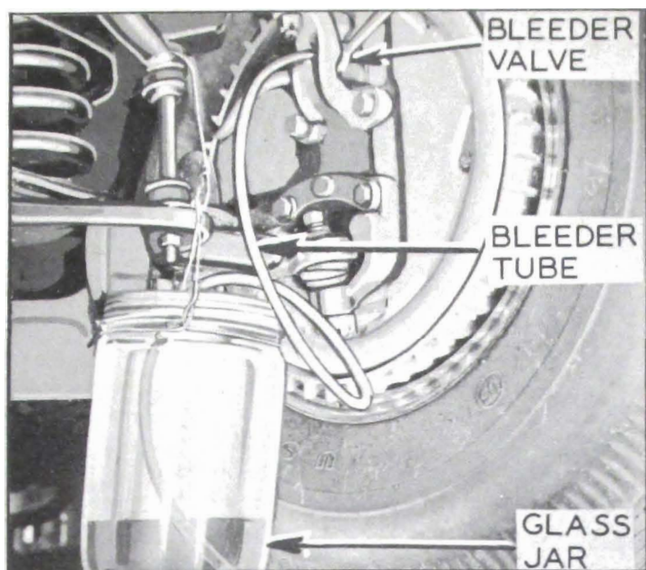
Figure 9-6—Bleeding Front Wheel Cylinder
