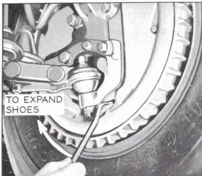
Figure 9-8—Expanding Brake Shoes
