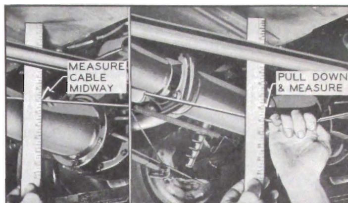
Figure 9-9—Checking Parking Brake Cable Adjustment
