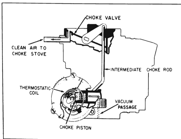
Figure 3-22—Choke System
