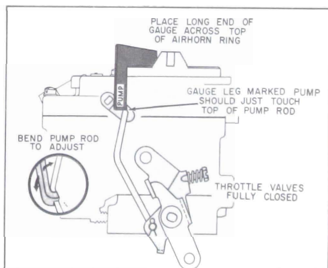
Figure 3-26—Pump Rod Adjustment
