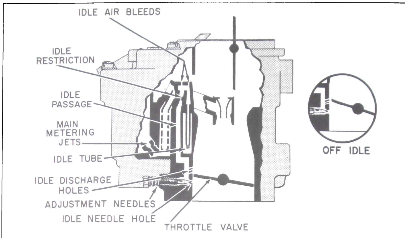
Figure 3-18—Low Speed System
