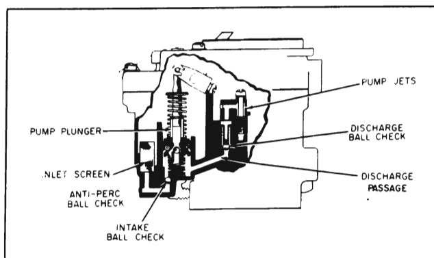
Figure 3-21—Accelerating Pump System
