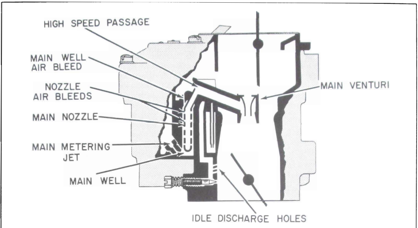
Figure 3-19—High Speed System
