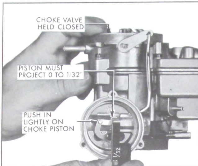
Figure 3-26A—Checking Choke Piston Adjustment
