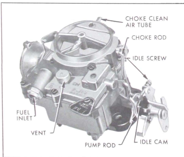
Figure 3-16—Rochester 2GC Carburetor Assembly
