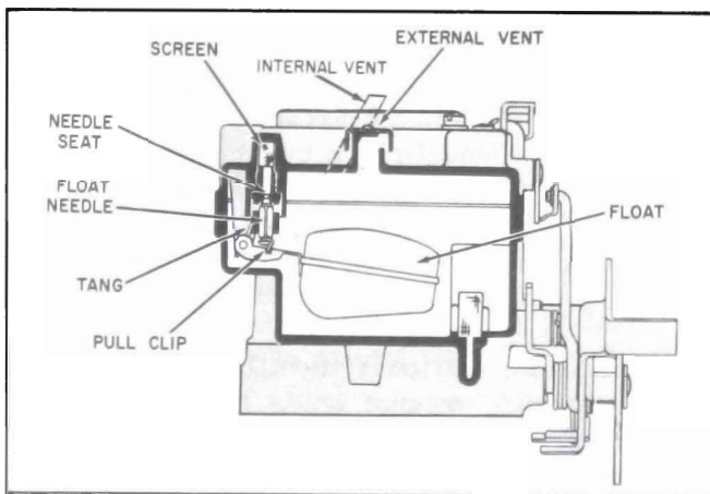
Figure 3-17—Float System
