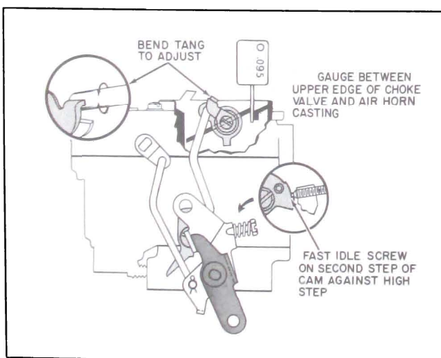
Figure 3-27—Choke Rod Adjustment
