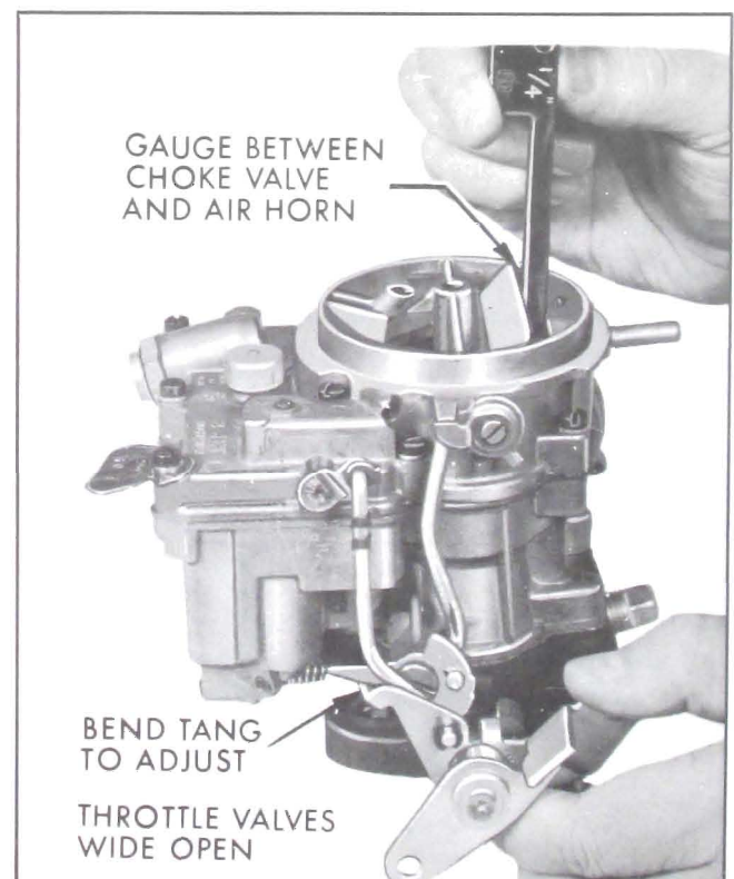
Figure 3-28—Choke Unloader Adjustment
