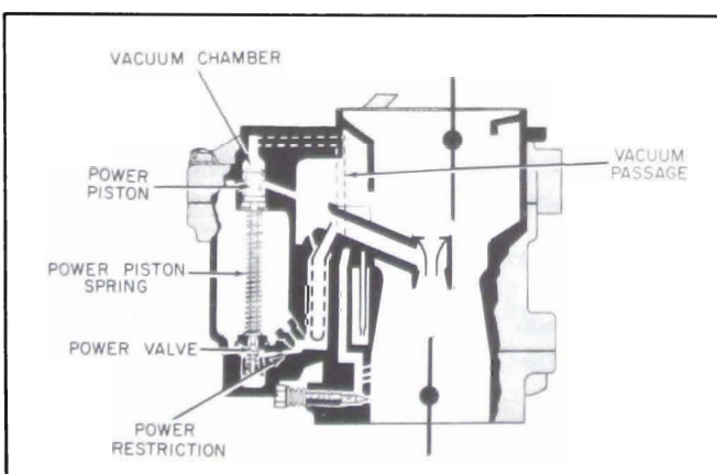
Figure 3-20—Power System
