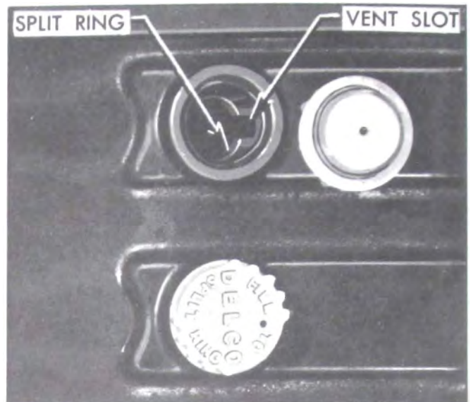
Figure 10-2—Battery Filler Well
