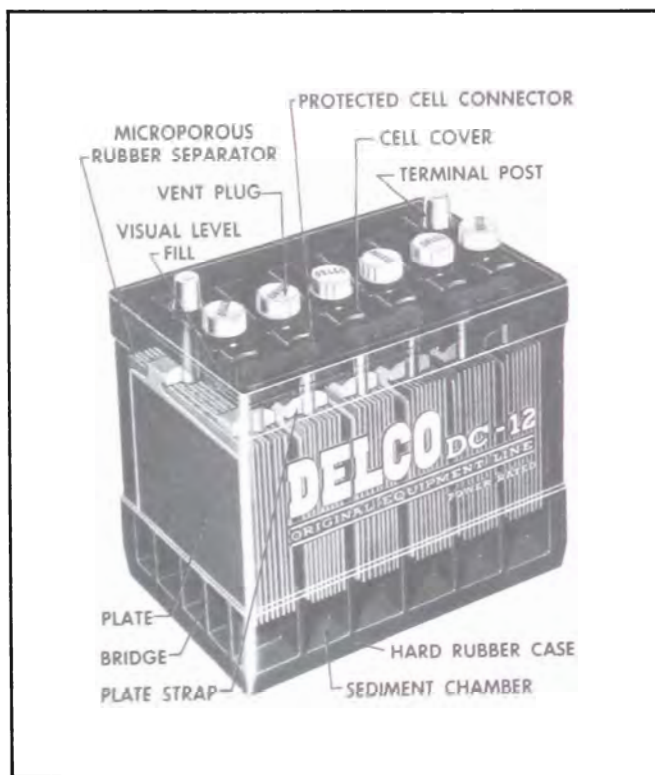
Figure 10-1—Battery
