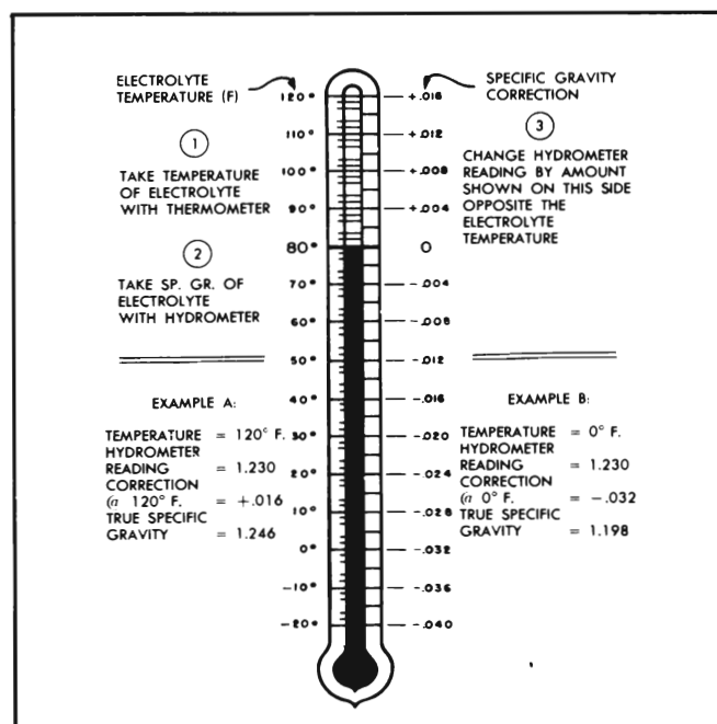
Figure 10-4—Specific Gravity Temperature Correction Scale
