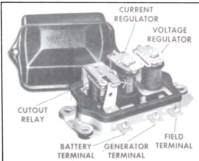
Figure 10-8—Generator Regulator
