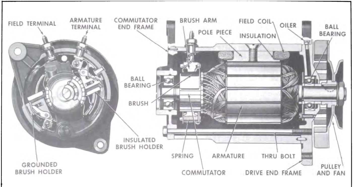
Figure 10-7—Generator, Sectional View
