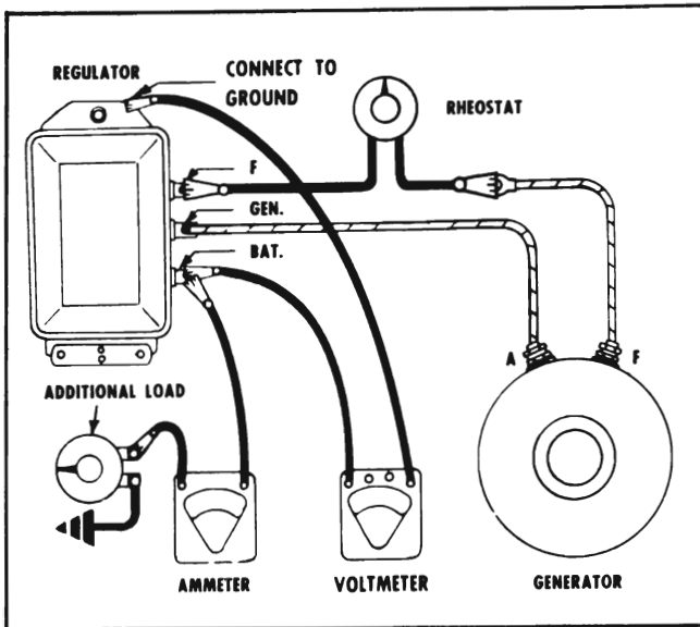
Figure 10-17—Testing Current Regulator
