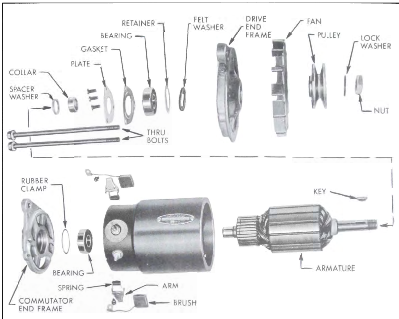
Figure 10-13—Generator Disassembled
