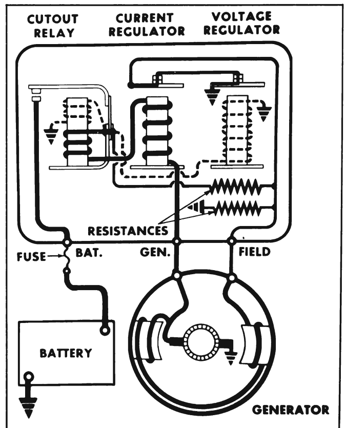
Figure 10-9—Generator System Circuits
