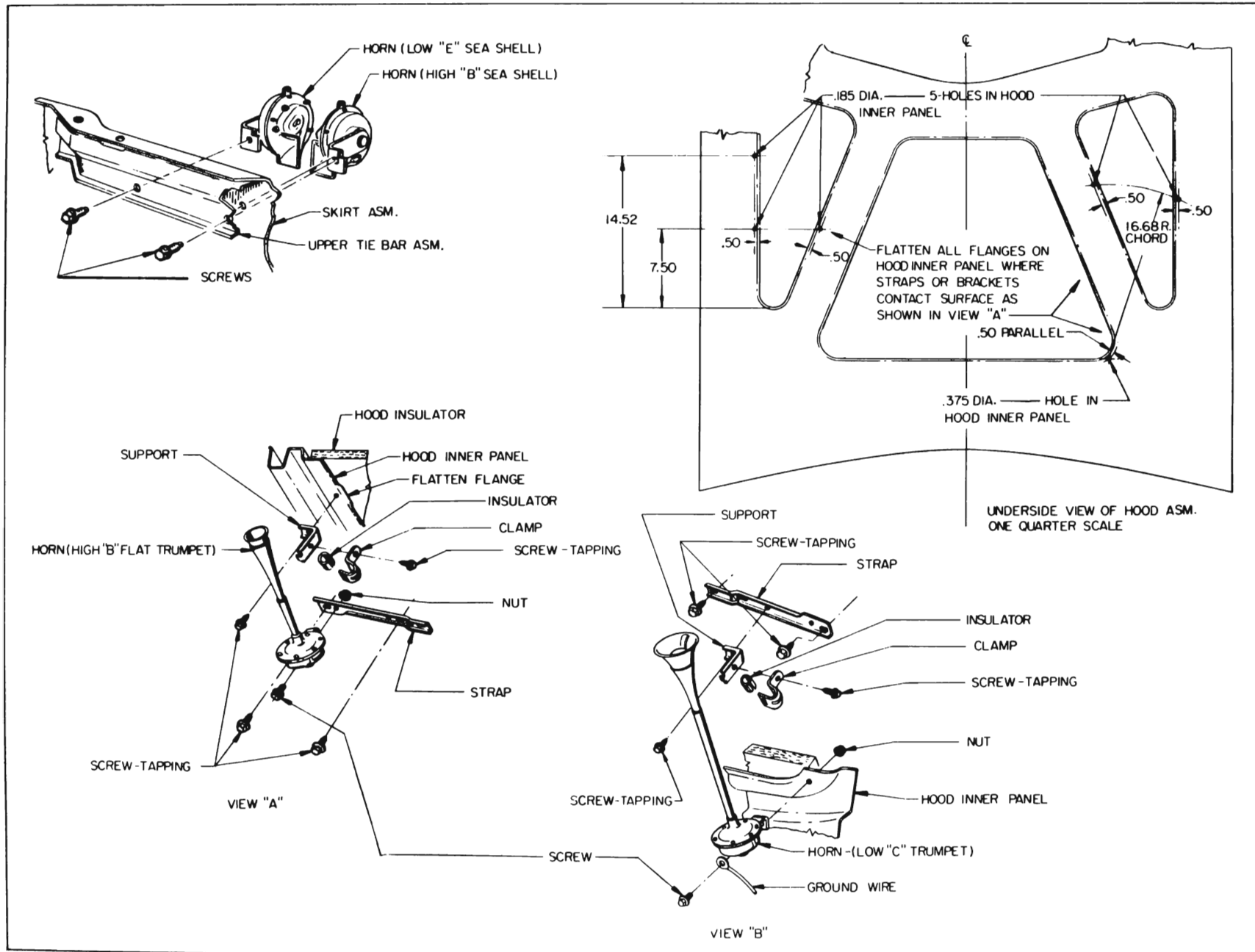
Figure 11-204—Four Note Horn Installation—4700 Series
