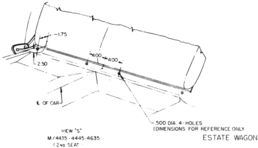
Figure 11-201—Seat Belt Installation—Illustration #6
