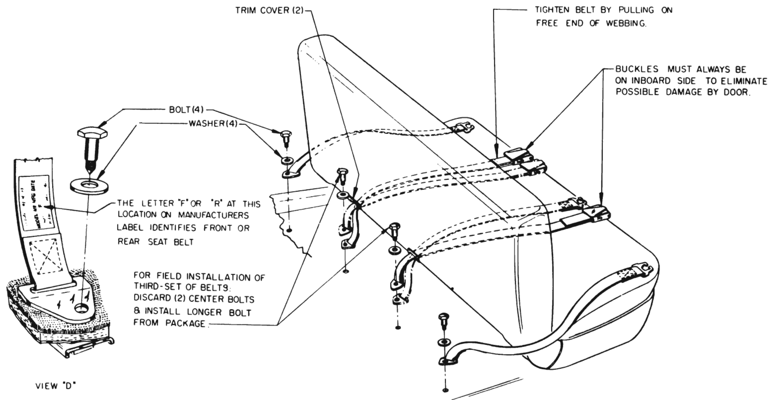
Figure 11-197—Seat Belt Installation—Illustration #2
