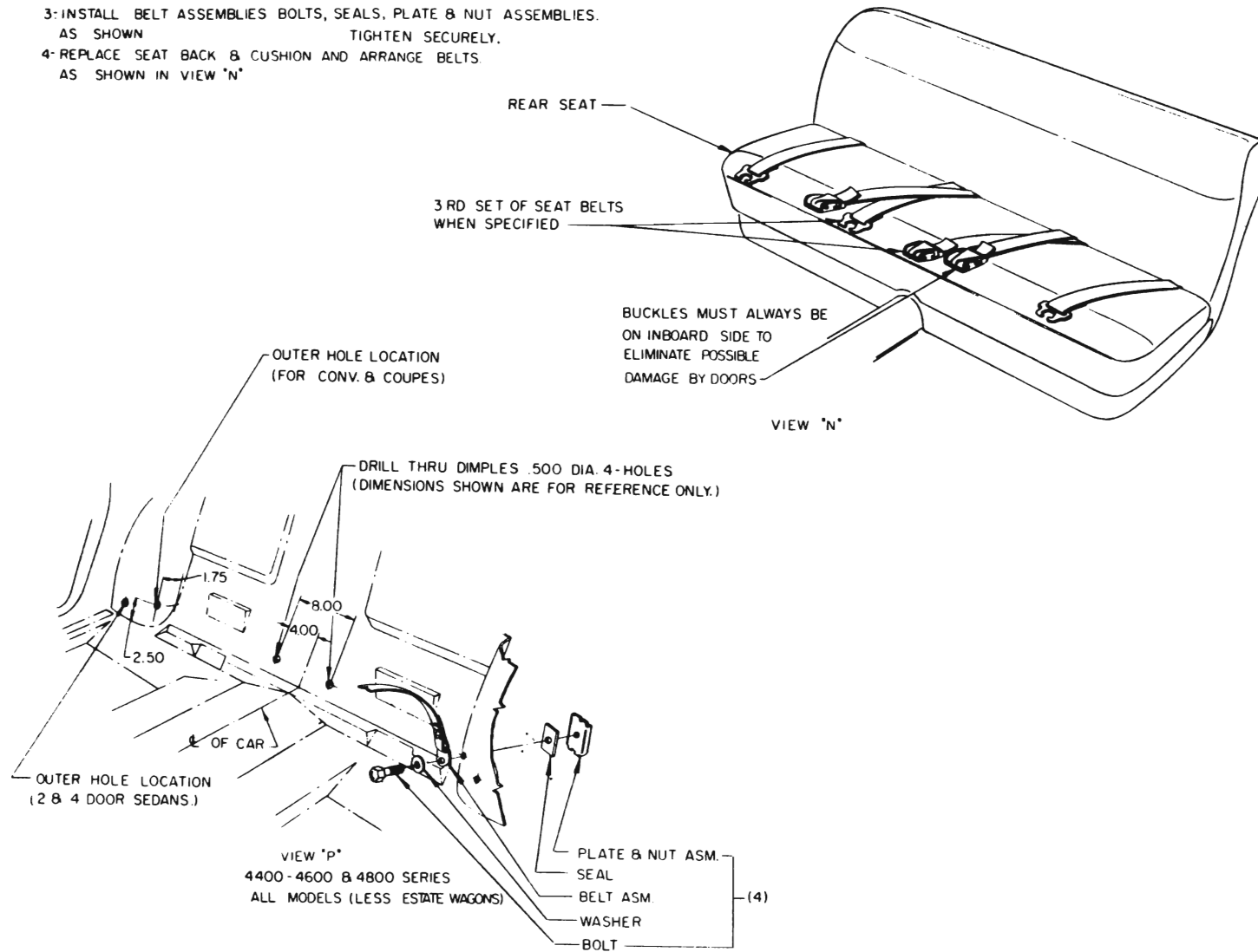
Figure 11-200—Seat Belt Installation—Illustration #5
