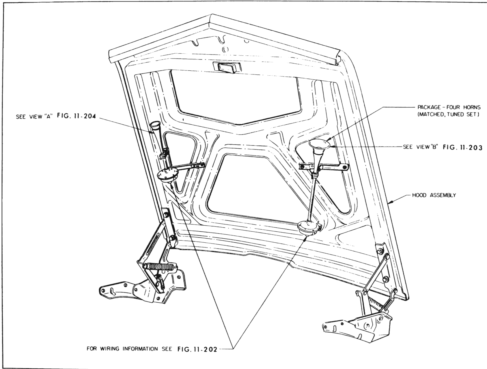
Figure 11-203—Four Note Horn Installation—4700 Series
