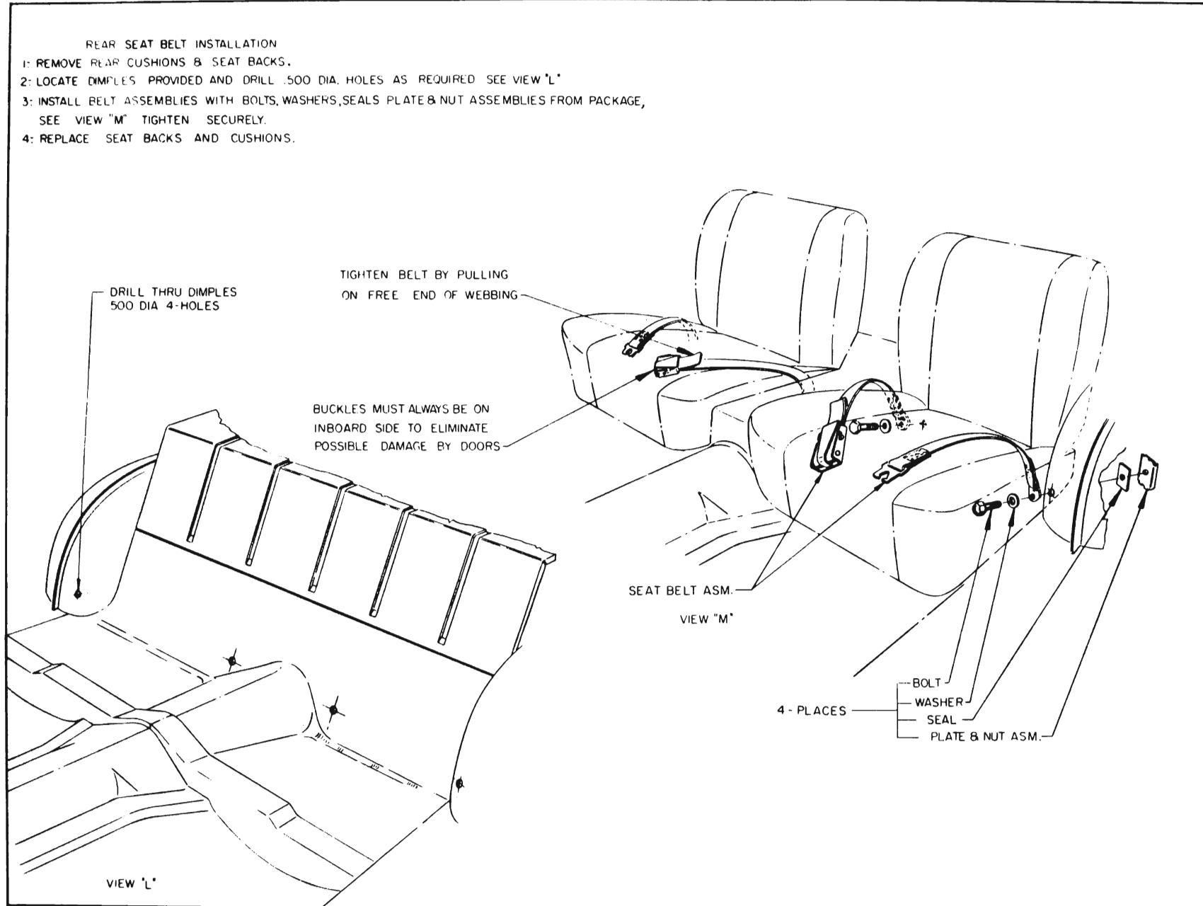
Figure 11-199—Seat Belt Installation—Illustration #4
