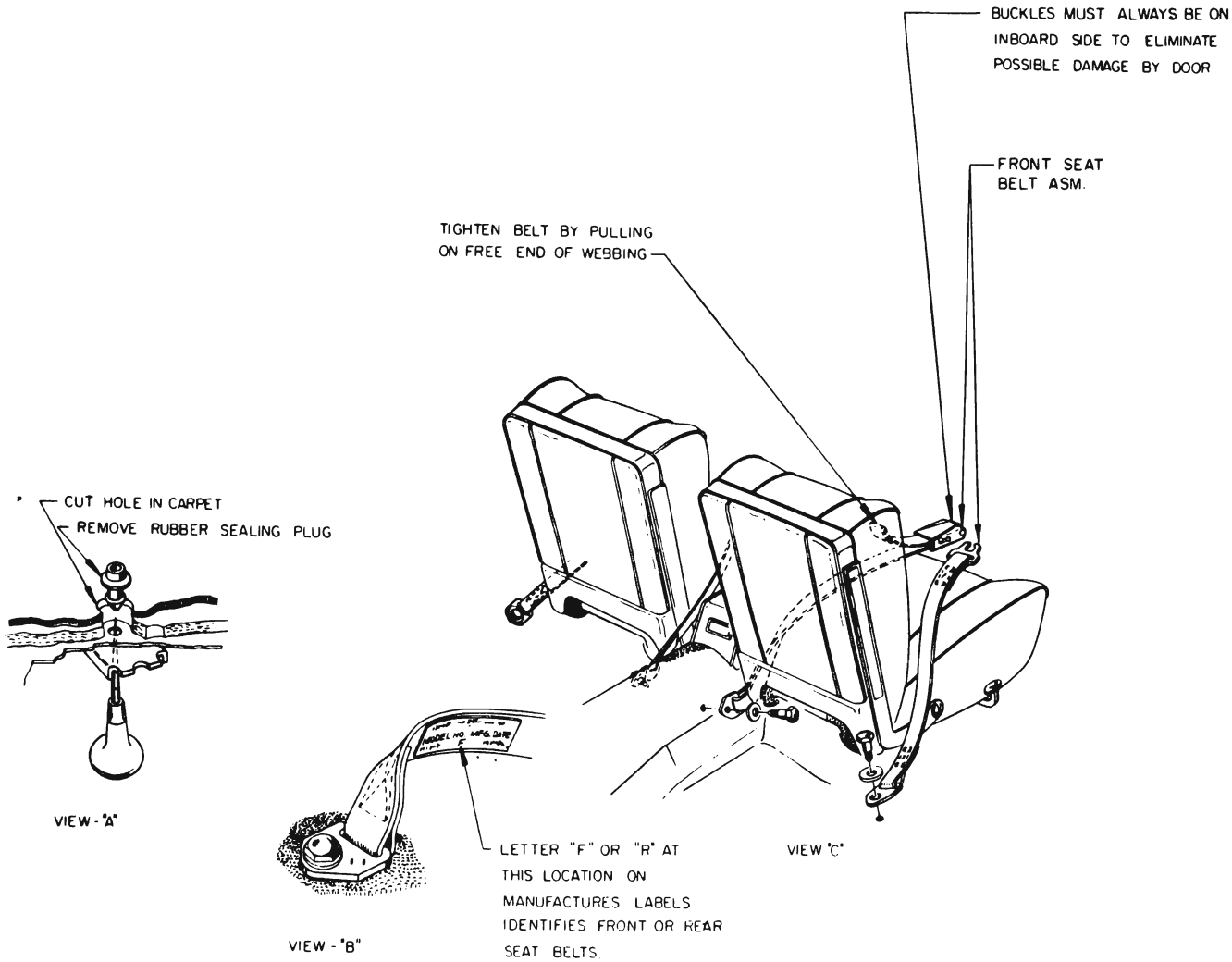
Figure 11-196—Seat Belt Installation—Illustration #1
