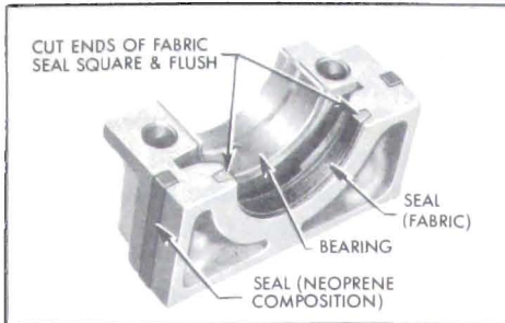
Figure 2-31—Rear Bearing Oil Seals
