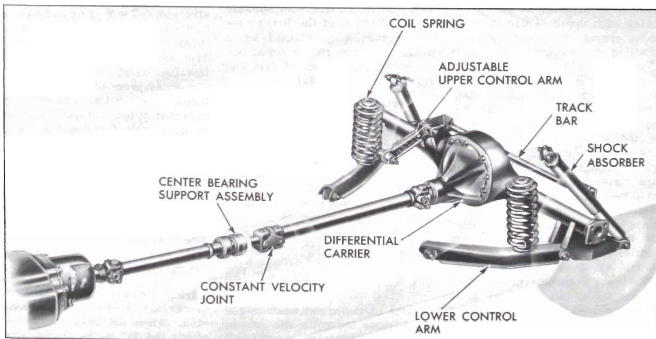
Figure 7-2—Rear Suspension
