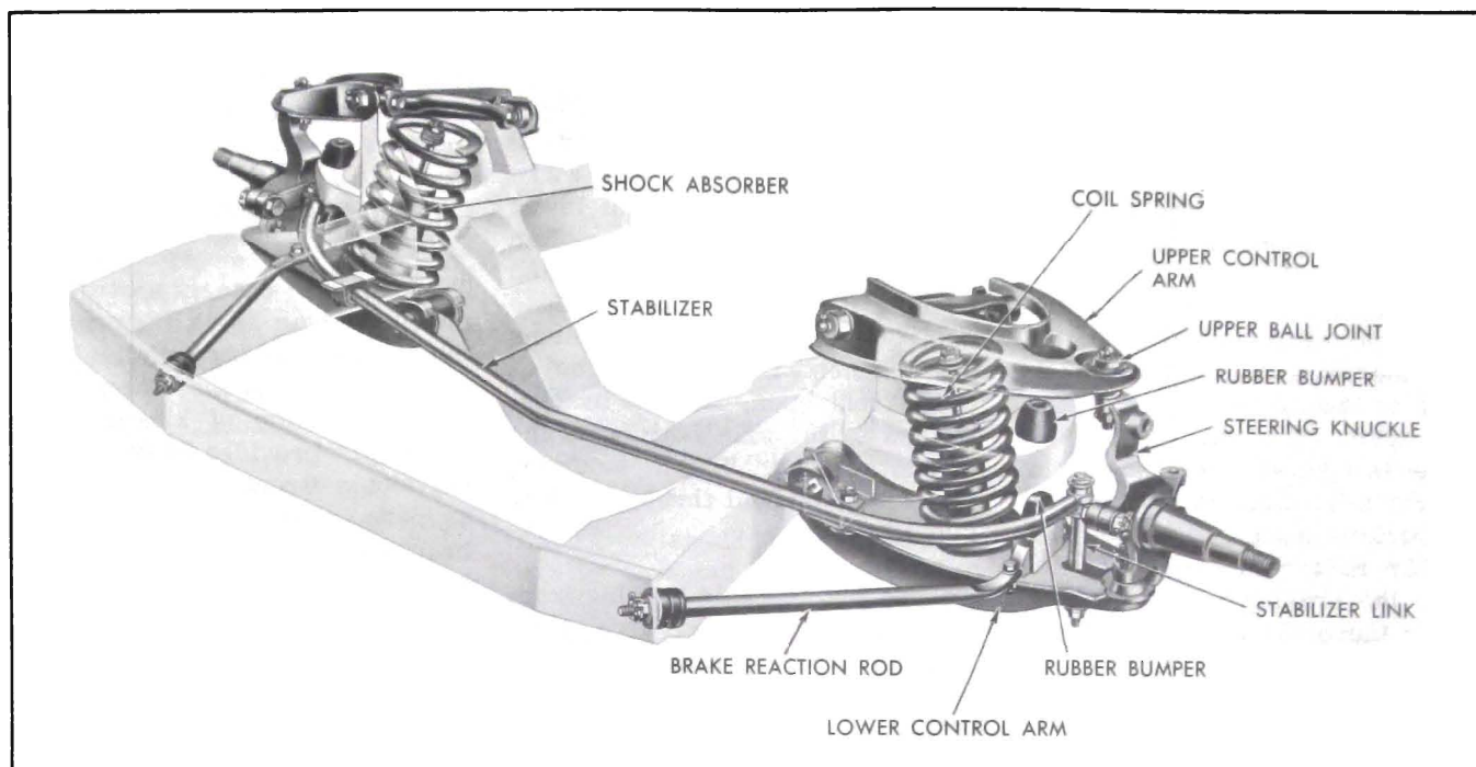
Figure 7-1—Front Suspension
