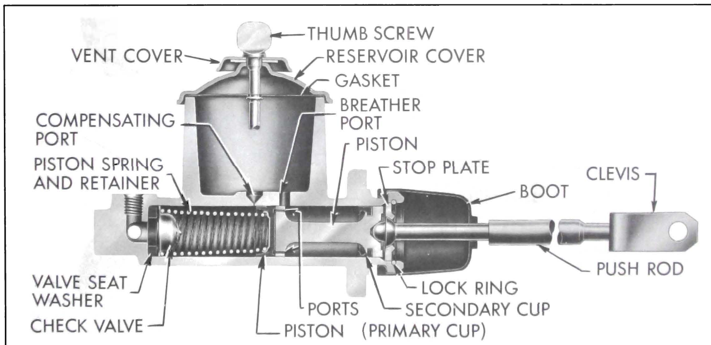
Figure 9-12—Brake Master Cylinder
