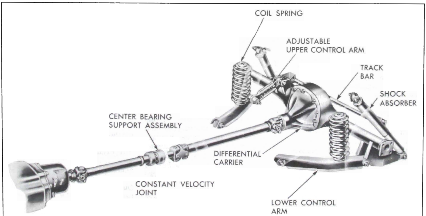
Figure 7-2—Rear Suspension
