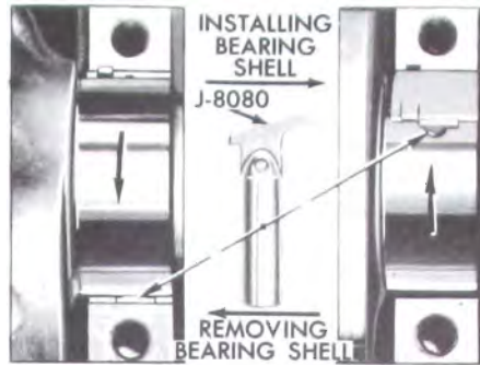
Figure 2-41—Removing and Installing Crankshaft Bearing Upper Shell
