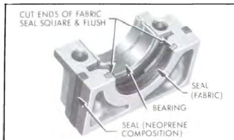
Figure 2-42—Rear Bearing Oil Seals
