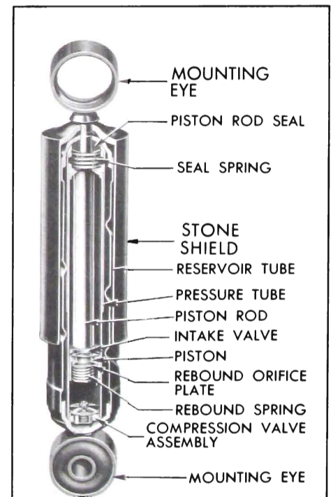
Figure 7-5—Typical Shock Absorber (Rear Shown)
