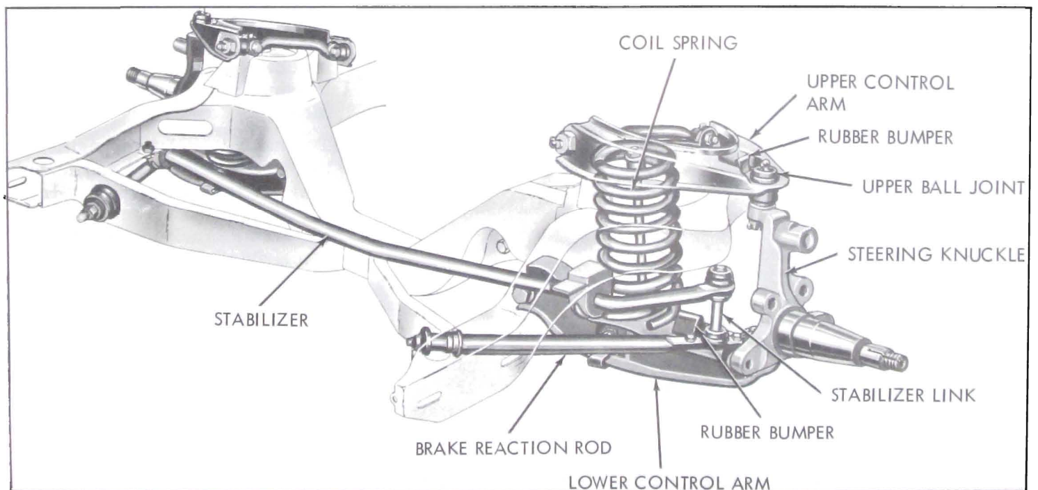
Figure 7-2—Front Suspension - 45, 46, 48000 Series
