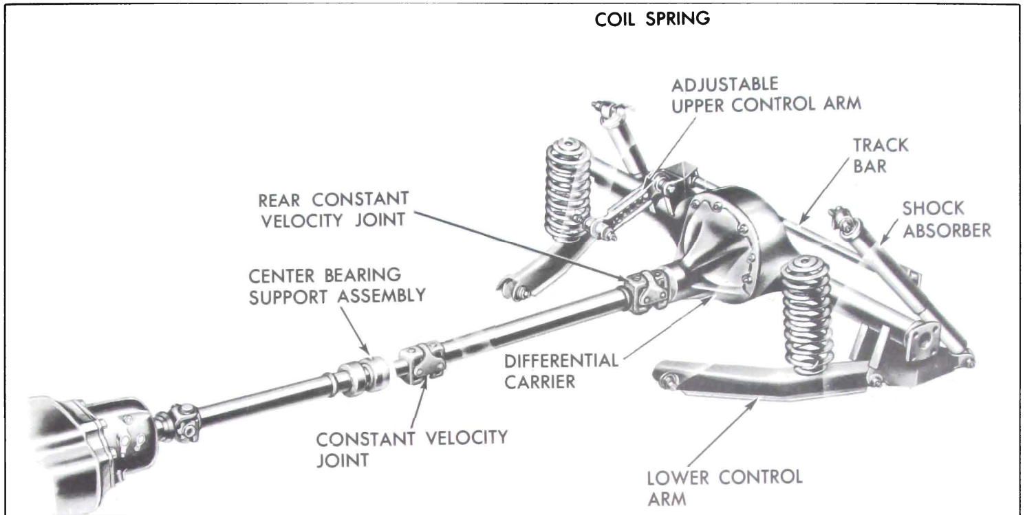
Figure 7-3—Rear Suspension - 49000 Series
