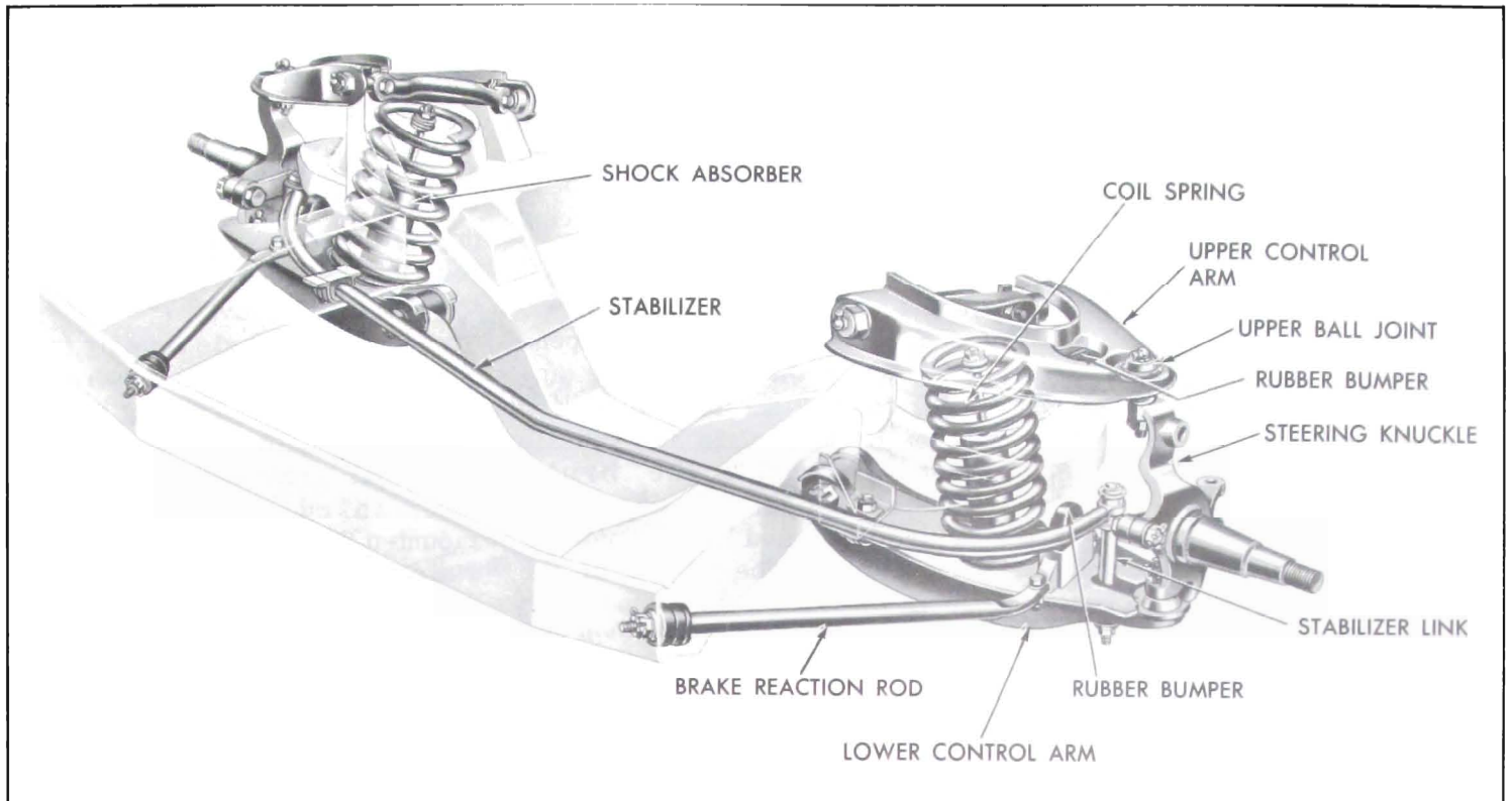
Figure 7-1—Front Suspension - 49000 Series
