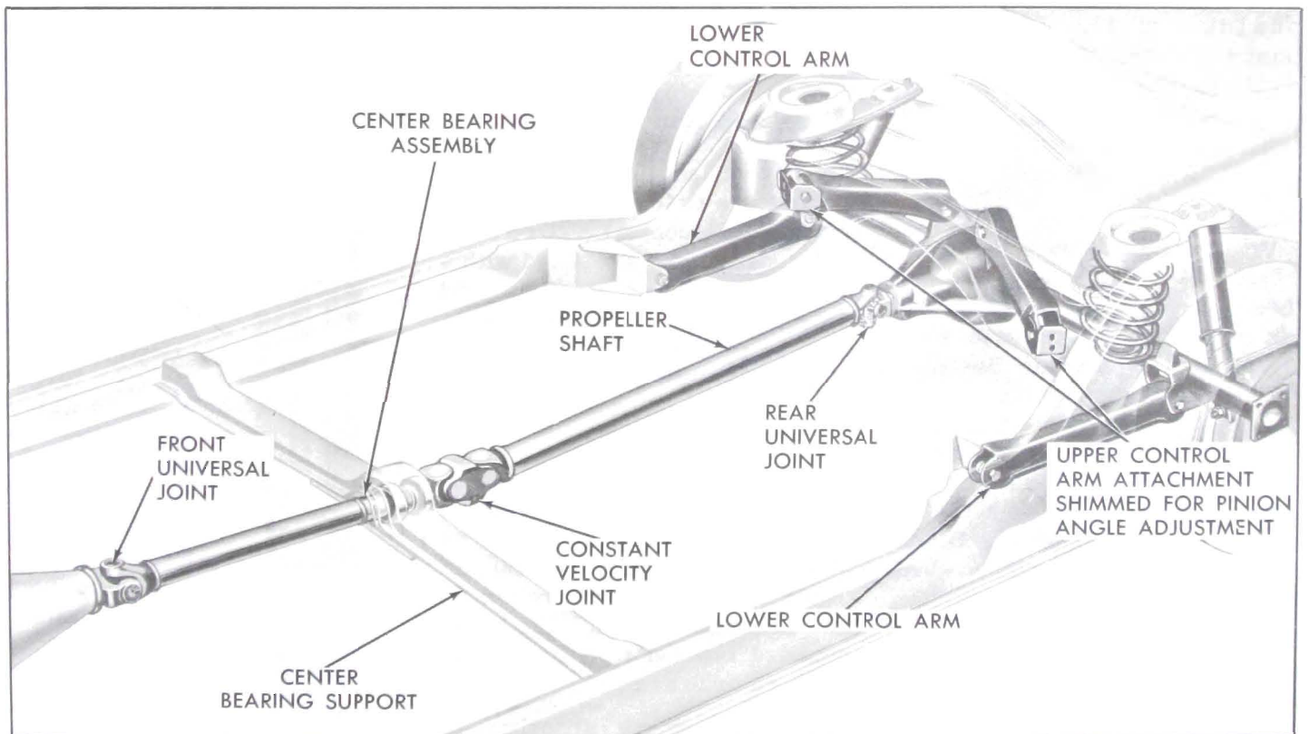
Figure 7-4—Rear Suspension - 45, 46, 48000 Series
